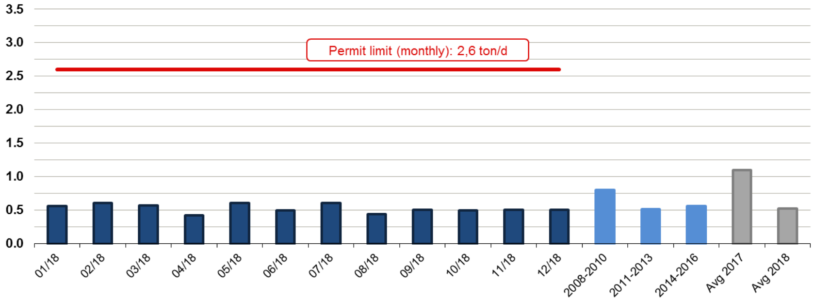
BOD 5 (DBO 5 ) - ton/d
