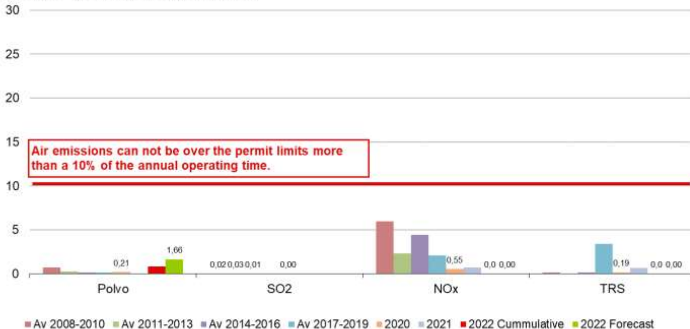
Lime kiln - % of time over permit limit
