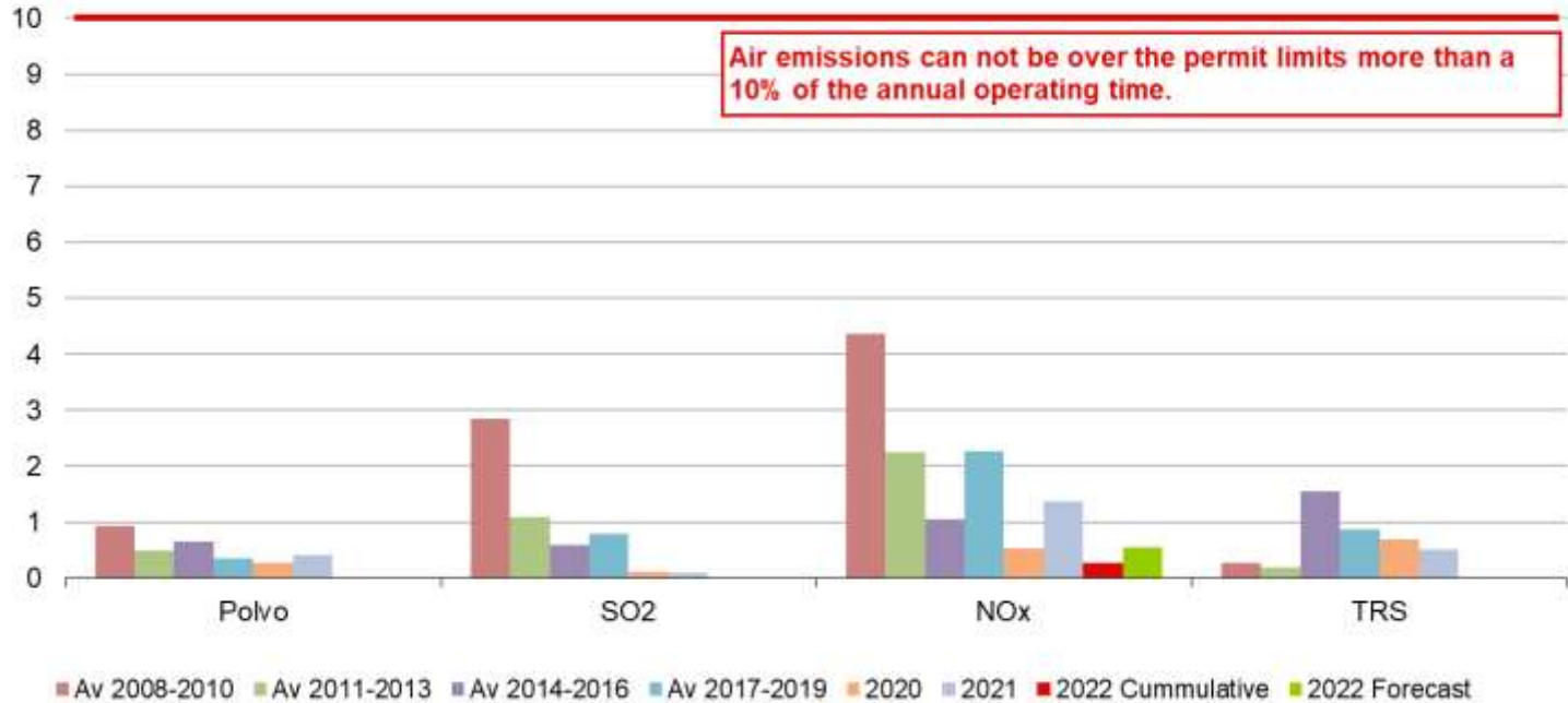
Boilers - % of time over permit limit
