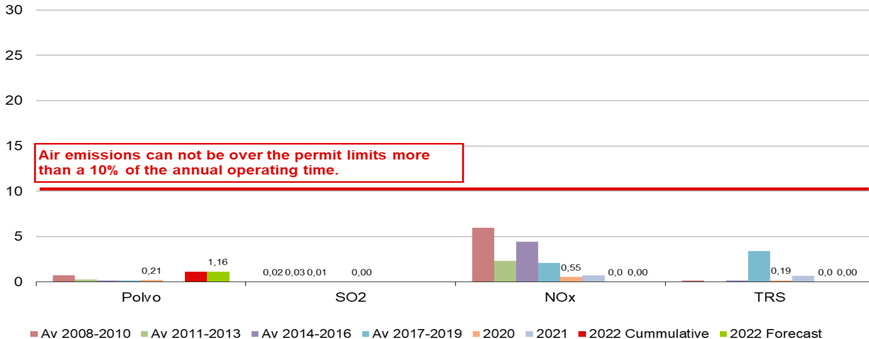
Lime kiln - % of time over permit limit
